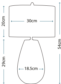
HARROW QN-HARROW-TL
