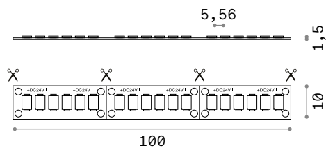
SMD 2835 180 LED/m
