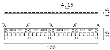
SMD 2835 240 LED/m
