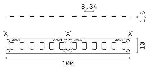
SMD 2835 120 LED/m
