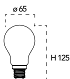
Lampada LED filamento 16W 230V
