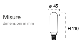
Lampada LED T45 8W 230V NDLS 360°
