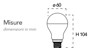
Lampada LED decorativa 7W 230V
